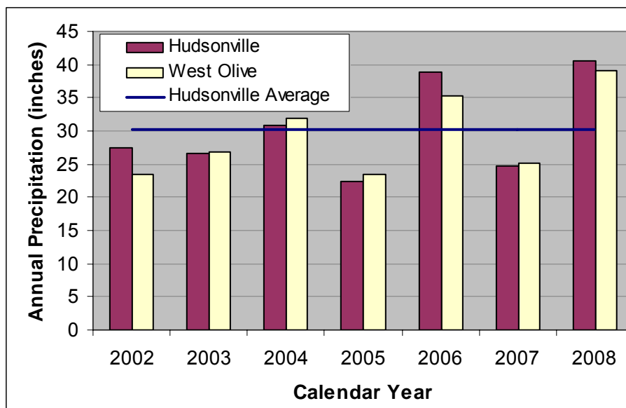
Figure 2 – Annual Precipitation
